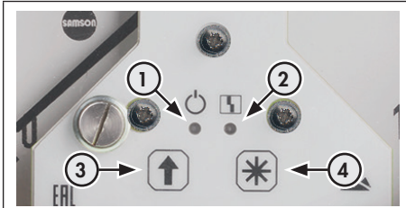
Fig. 11: Operating controls
