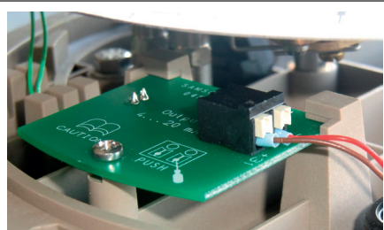
Fig. 10: Connecting the measuring signal lines on the terminal board
